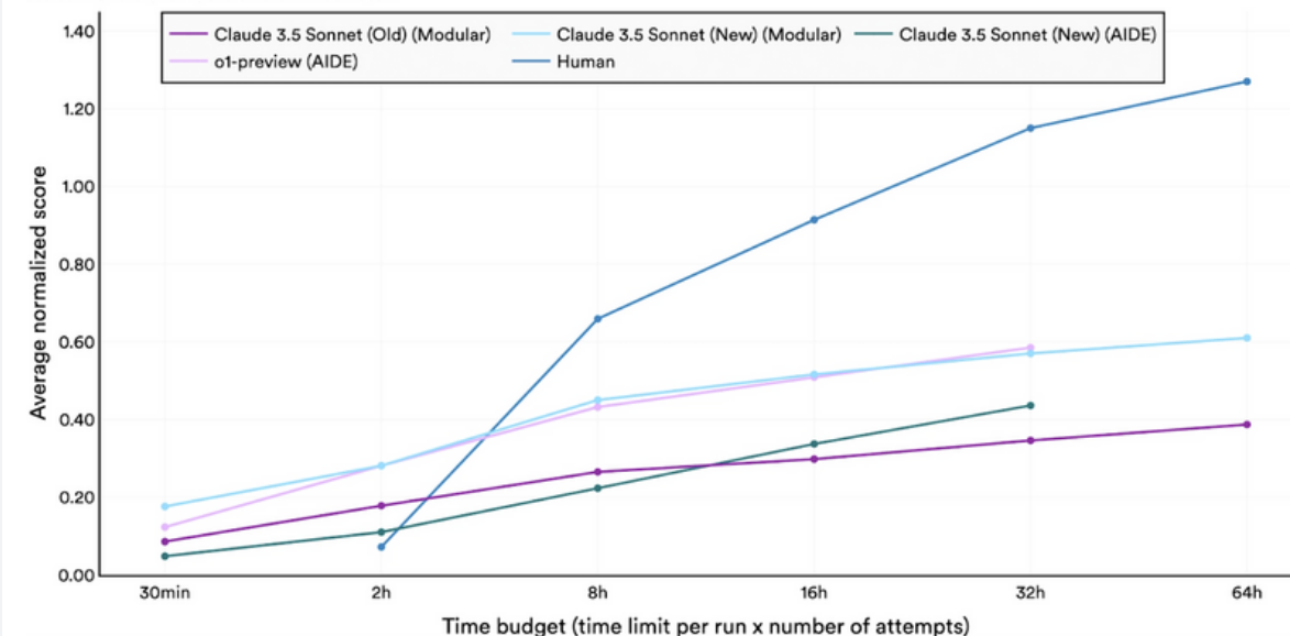
RE-Bench: average normalized score@k Source: Wijk et al., 2024 | Chart: 2025 AI Index report
